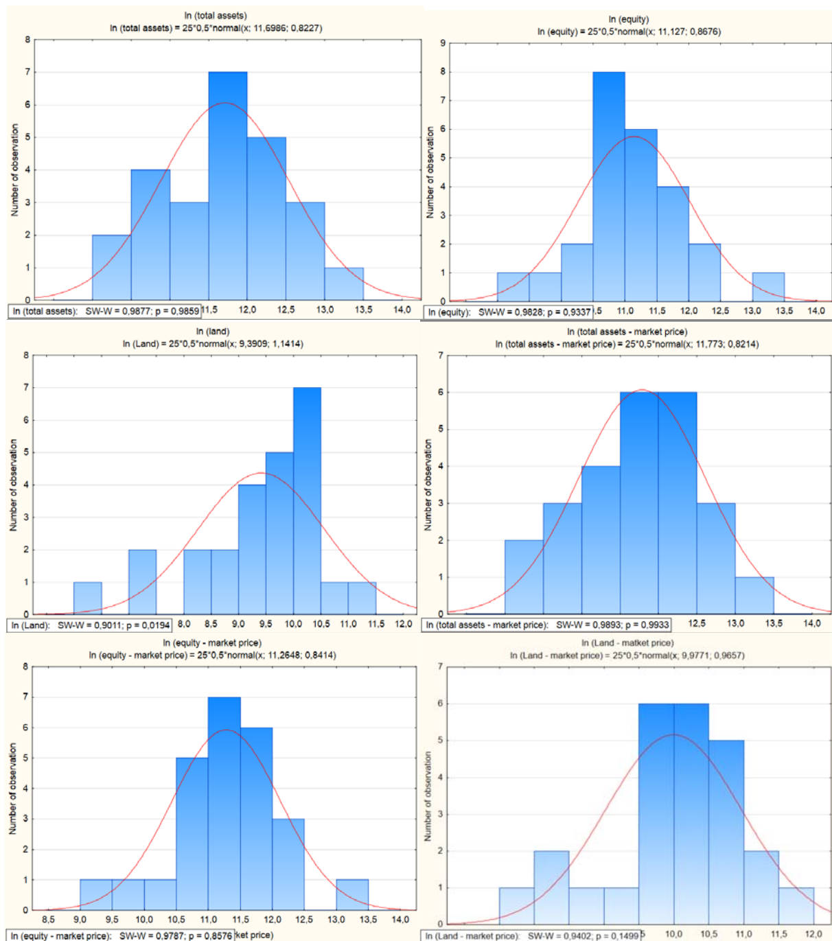
Fig. 4 Result of the normality test (land valuation) – a normal distribution
