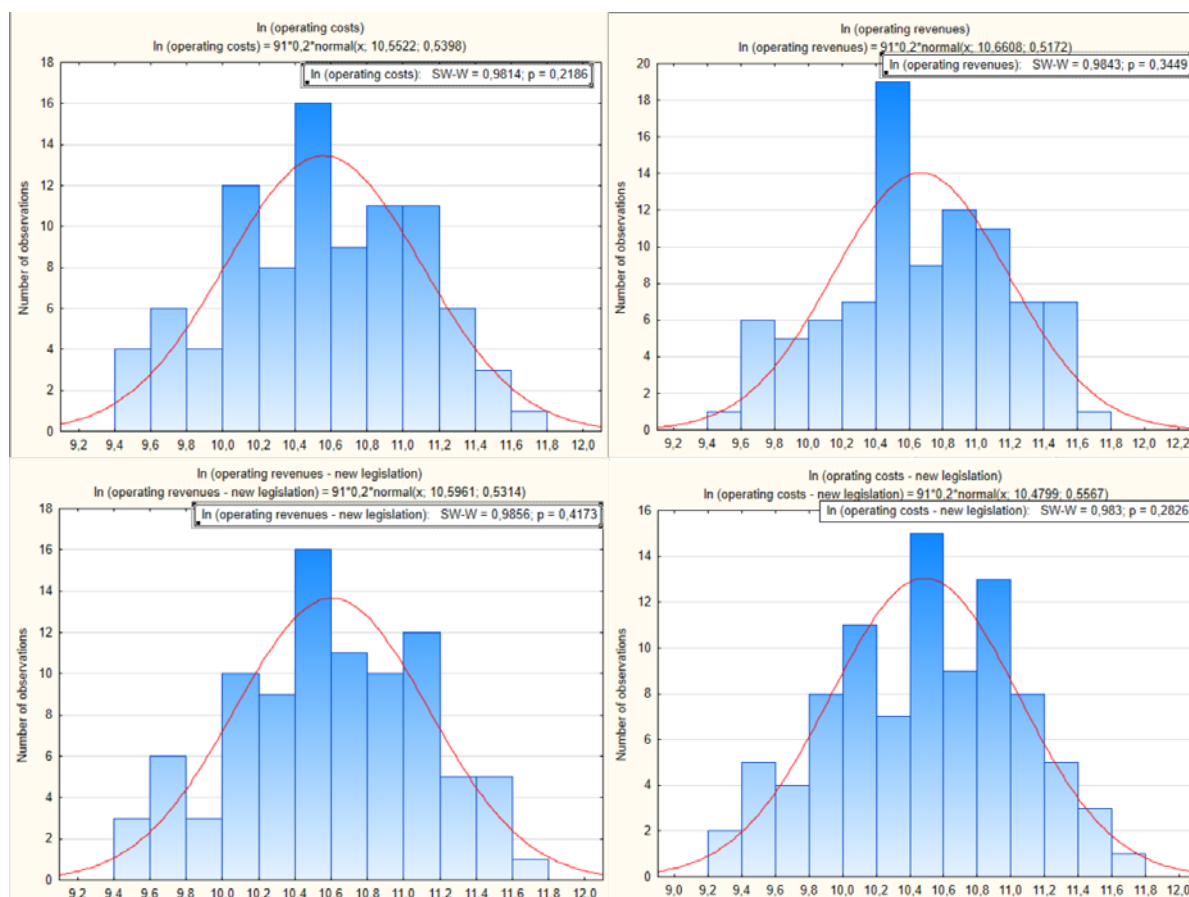
Fig. 9 Result of the normality test for transformed variables (internally produced inventory and in capitalization) – a normal distribution
