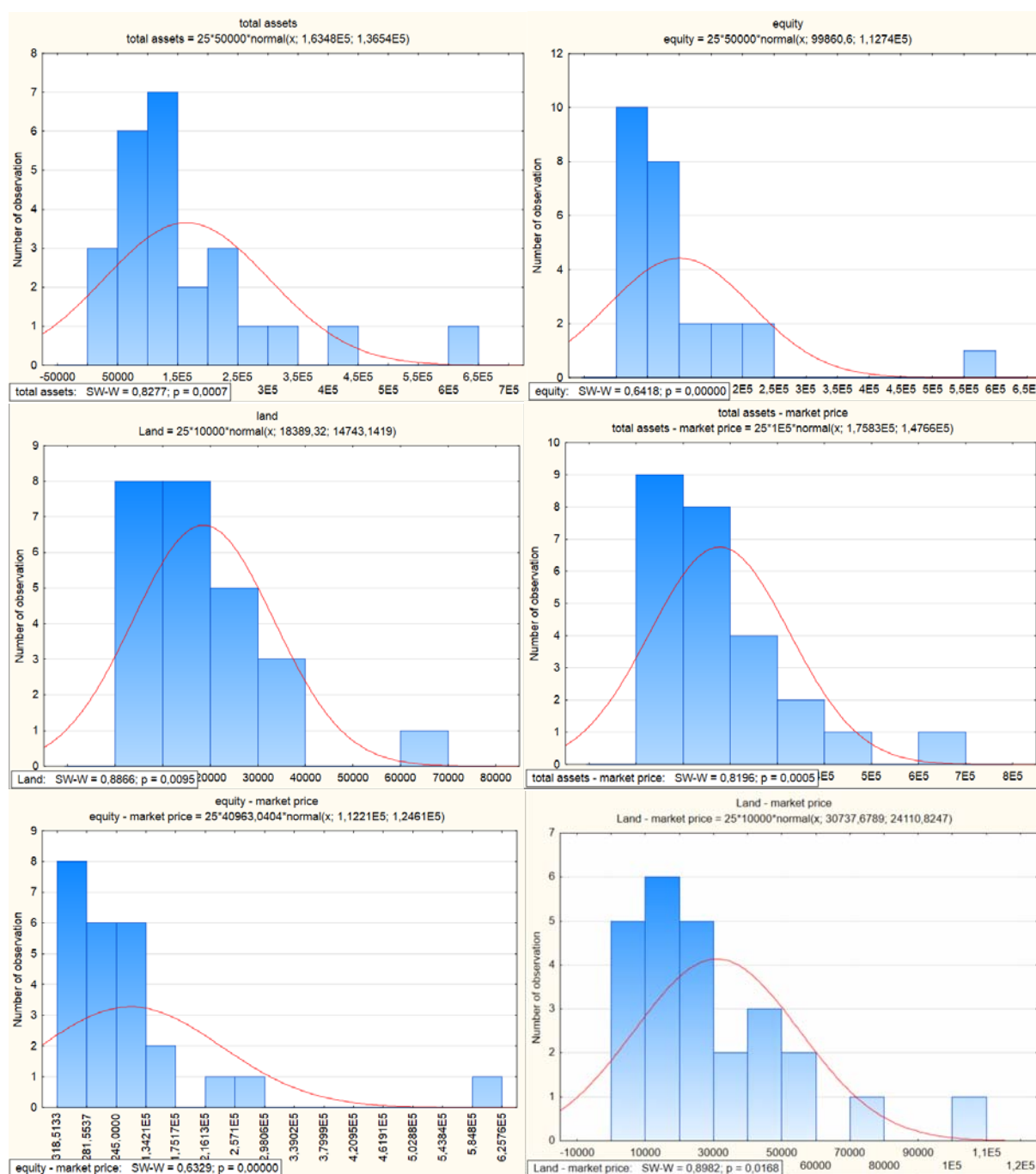
Fig. 3 Result of the normality test (land valuation) – not a normal distribution
