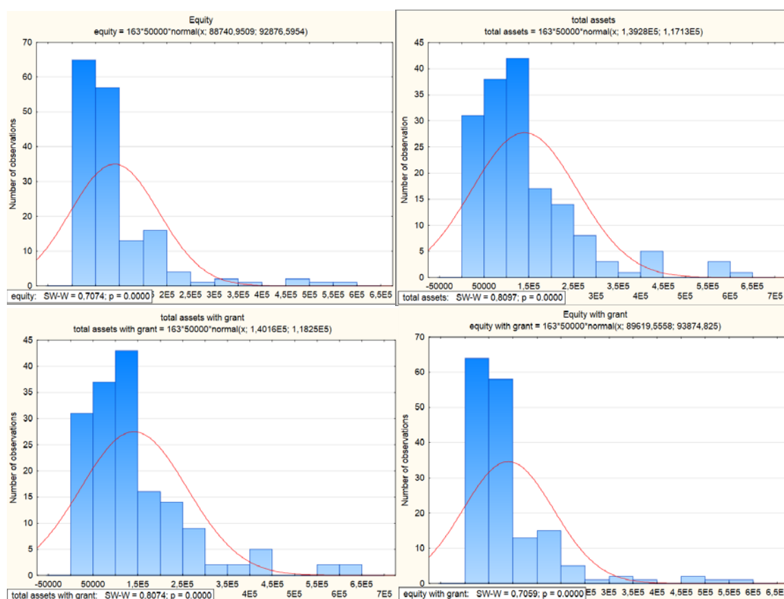
Fig. 1 Result of the normality test (investment subsidy) – not a normal distribution
